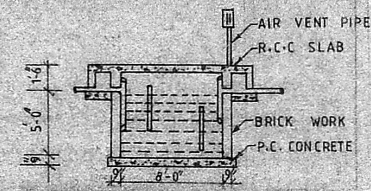
SECTION ON SEPTIC TANK
