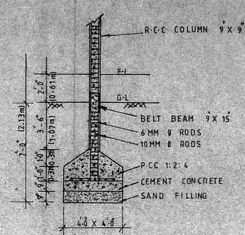
SECTION ON R.C.C. COLUMN
